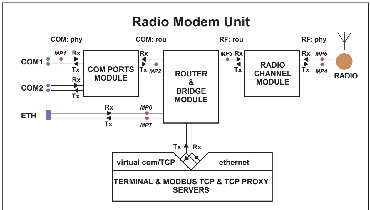
Fig. 7.13: Interfaces
