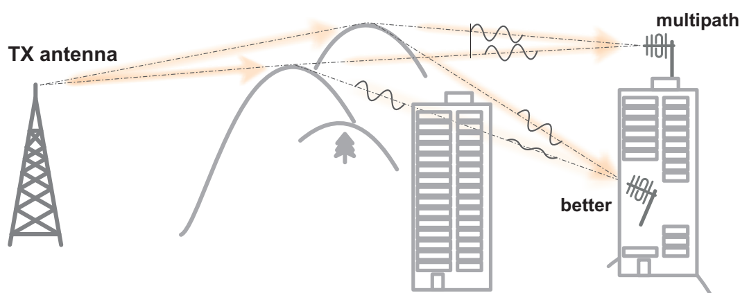
Fig. 3.4: Antenna location
