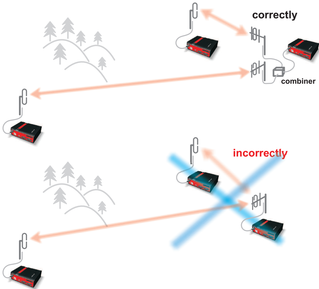
Fig. 3.5: Main lobe
