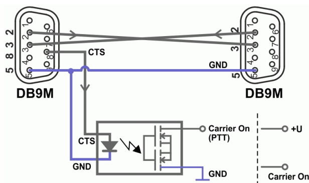
Fig. 4.34: Cable connection
