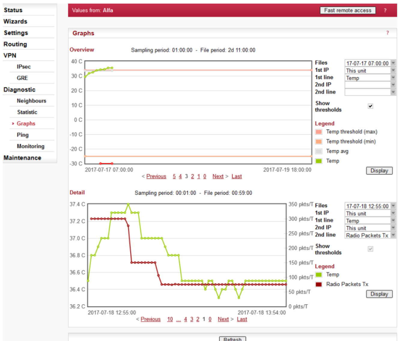
Fig. 7.11: Menu Graphs
