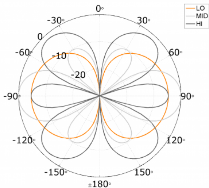
Typical Normalized Radiation Pattern
