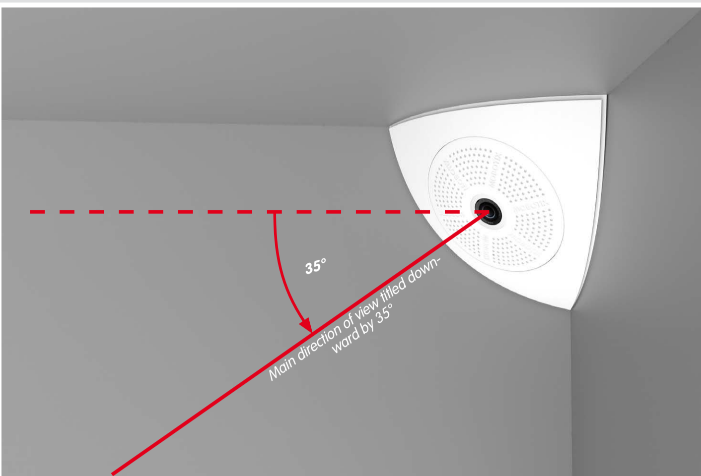
Set for corner installation of MOBOTIX cameras c25 (not included), allows elegant installation of the cameras in corners
